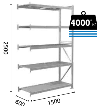
MS Pro 250/150x60/5
